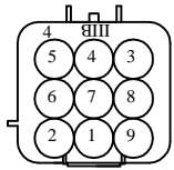
DJK7091-2.3-11 9Pin Male (See from input side)
