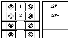
Dual KLS-8080I/IPS Controller Assembly Wiring Diagram
