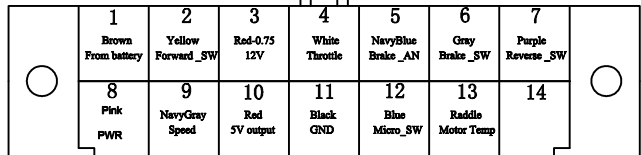
KLS-D Controller Assembly Wiring Diagram
