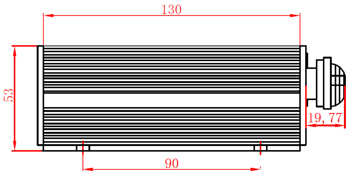
Fig.2 (Side view)
