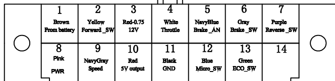
14PIN Connector
